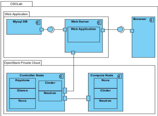
Figure 3 – System components
